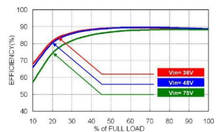
DFEC60-48S05 Efficiency vs. Output Load
