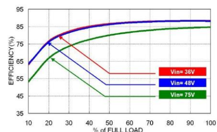
DFED20-48S05 Efficiency vs. Output Load
