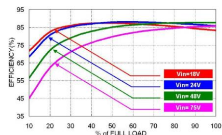
DFED20-48S05W Efficiency vs. Output Load
