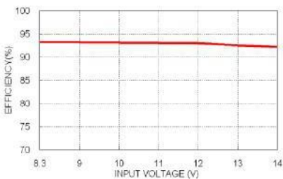
DOS10-12T, Vout=3.3V Efficiency vs. Input Voltage
