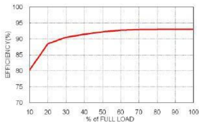
DOS10-12T, Vout=3.3V Efficiency vs. Output Load
