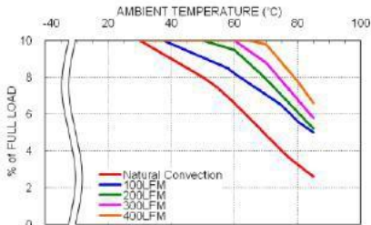
DOS10-12T, Vout=3.3V Derating Curve
