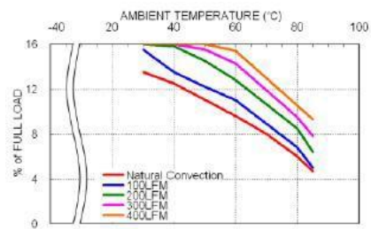
DOS16-05T, Vout=3.3V Derating Curve
