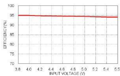
DOS16-05T, Vout=3.3V Efficiency vs. Input Voltage
