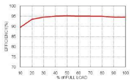
DOS16-05T, Vout=3.3V Efficiency vs. Output Load
