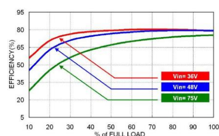
EDL03-48S05 Efficiency vs. Output Load
