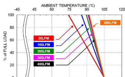
EDL03-24S05W Derating Curve
