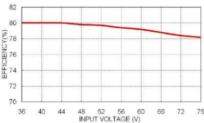
FDC05-48S05 Efficiency vs. Input Voltage
