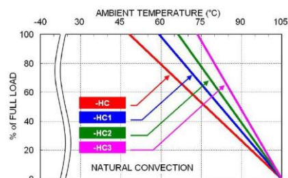
FED60-48S12 Derating Curve With Heat-sink
