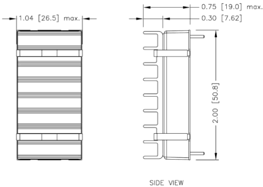
FED60-□□□□W- HC1 7GA0120P01-F
