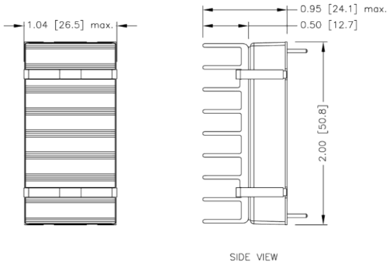
FED60-□□□□W- HC2 7GA0121P01-F
