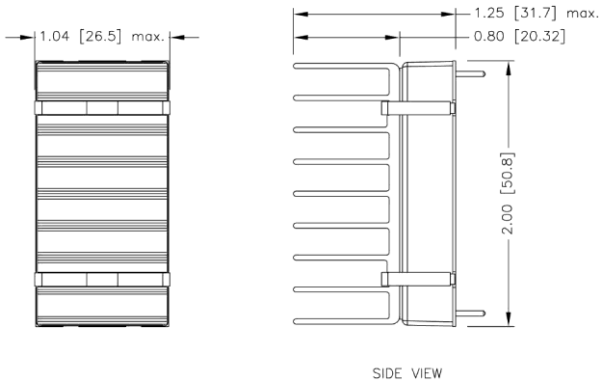
FED60-□□□□W- HC3 7GA0122P01-F
