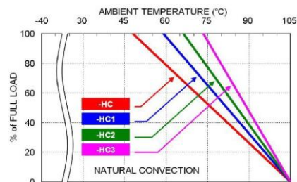
FED60-48S12W Derating Curve With Heat-sink
