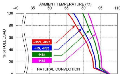
HAE100-48S05W Derating Curve with Heat-sink (See Thermal Considerations)
