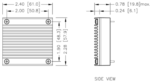
HAE150-□□S□□- HS2 7G-0023A-F
