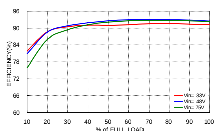
HAE150-48S05 Efficiency vs. Output Load
