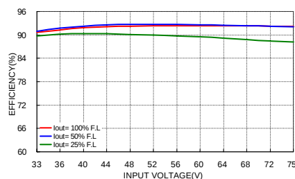
HAE150-48S05 Efficiency vs. Input Voltage
