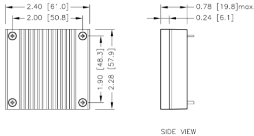
HAE150-□□S□□- HS1 7G-0022A-F
