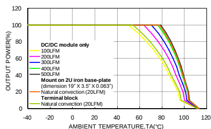
HAE150-48S05 Derating Curve (See Thermal Considerations)
