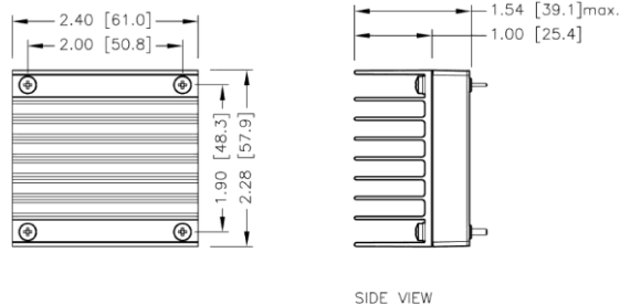
HAE150-□□S□□- HS5 7GA0128P01-F
