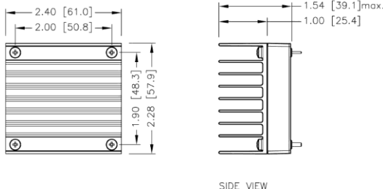
HAE150-□□S□□W- HS5 7GA0128P01-F
