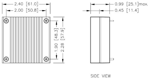
HAE150-□□S□□W- HS3 7G-0024A-F
