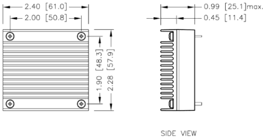
HAE150-□□S□□W- HS 7G-0021A-F
