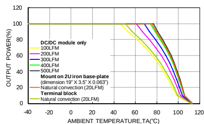
HAE150-48S05W Derating Curve (See Thermal Considerations)
