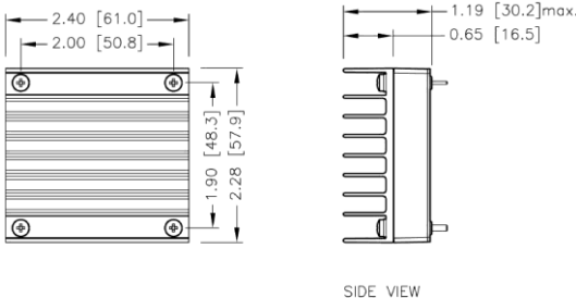
HAE150-□□S□□W- HS4 7GA0127P01-F
