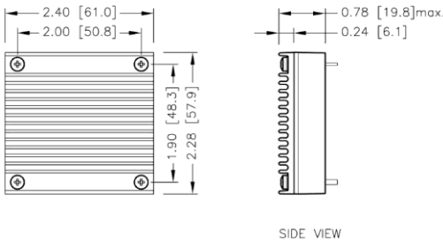
HAE150-□□S□□W- HS2 7G-0023A-F
