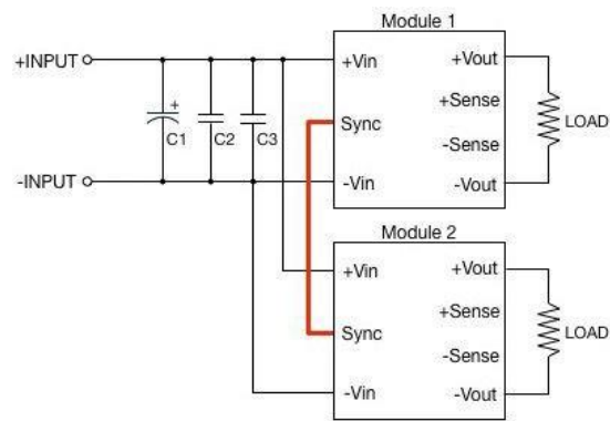
Synchronous Circuits
