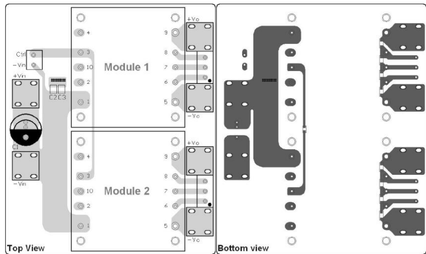
Recommended Layout
