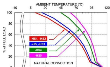
HAE200-48S05 Derating Curve with Heat-sink (See Thermal Considerations)
