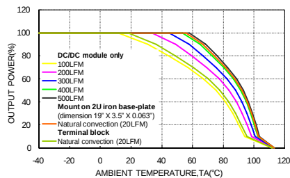
HAE200-48S05 Derating Curve (See Thermal Considerations)
