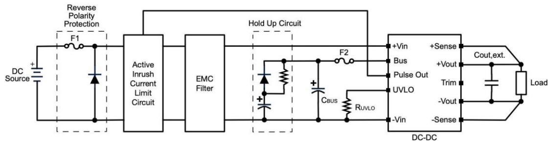
Typical Connection
