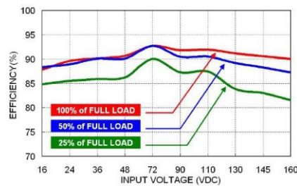
HAE200-72S12UA Efficiency vs. Input Voltage
