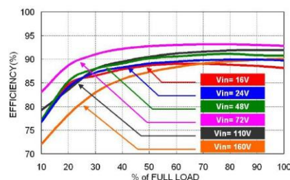
HAE200-72S12UA Efficiency vs. Output Load
