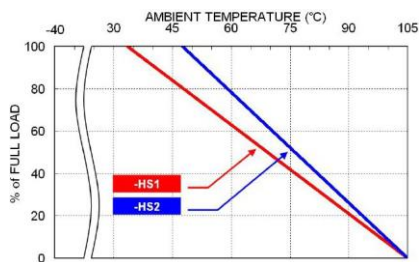
HAE200-72S12UA Derating Curve with Heat-sink (See Thermal Considerations)
