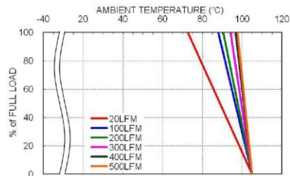
LCD15-48S05 Derating Curve With Heat-sink
