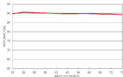
LCD20-48S05W Efficiency vs. Input Voltage
