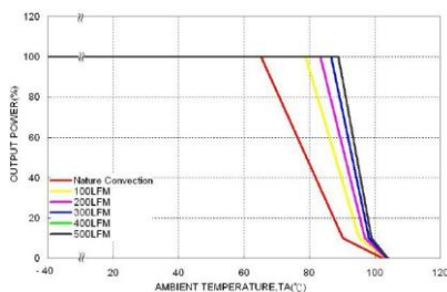
LCD20-48S05W Derating Curve
