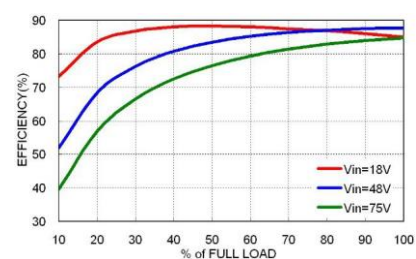
LED15-48S05W Efficiency vs. Output Load
