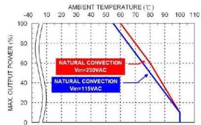
Derating Curve vs. Ambient Temperature MAC15USxxB xx=3P3/05/7P5/09/12/15/18 Connector Option : (-M / -T / -D)
