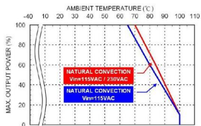
Derating Curve vs. Ambient Temperature MAC15USxxB xx=24/28/36/48/53 Connector Option : (-M / -T / -D)
