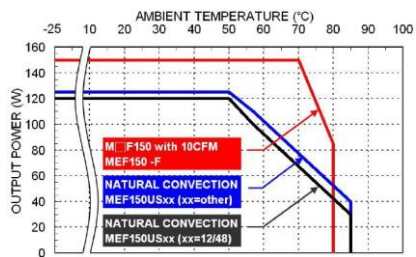
Derating Curve vs. Ambient Temperature Vin=115VAC
