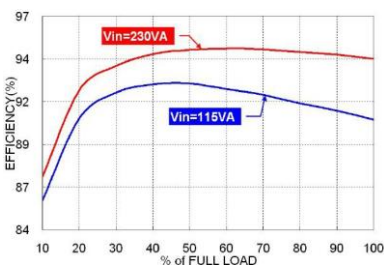
Efficiency vs. Output Load MAH450US24 with Forced air cooling
