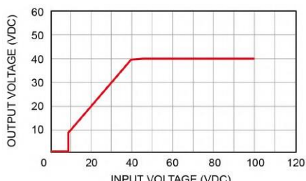
Transfer Function
