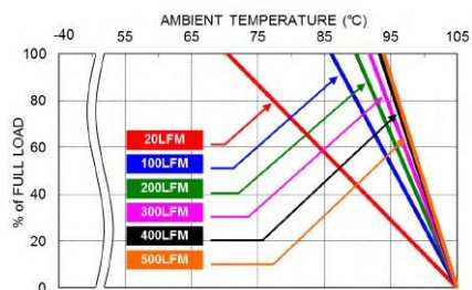
Derating Curve
