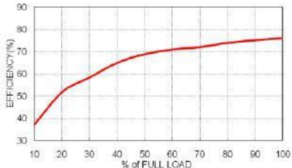
MKC03-48S05 Efficiency vs. Output Load
