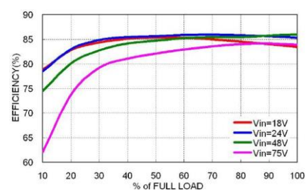
MOP10-48S05WA Efficiency vs. Output Load
