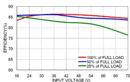
MOP10-48S05WA Efficiency vs. Input Voltage
