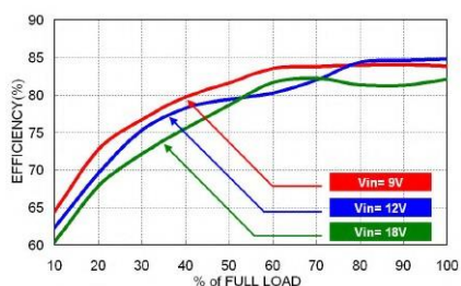
MPL02-12S12 Efficiency vs. Output Load
