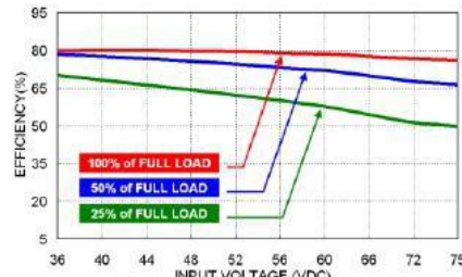
MPS(H)04-48S05 Efficiency vs. Input Voltage
