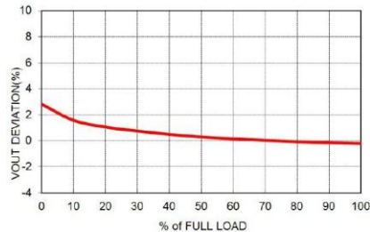
MPU01-24S05 Vout Deviation vs. Output Load
