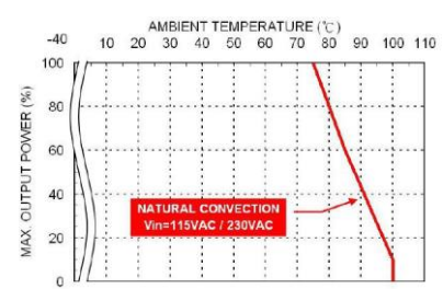
Derating Curve vs. Ambient Temperature MSC15USxxB xx=24/28/36/48/53 Connector Option : (-M / -T / -D)
