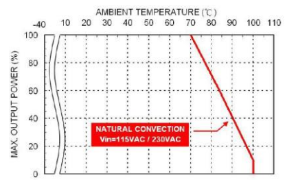
Derating Curve vs. Ambient Temperature MSC15USxxB xx=3P3/05/7P5/09/12/15/18 Connector Option : (-M / -T / -D)
