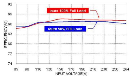
MSC15US12B Efficiency vs. Input Voltage
