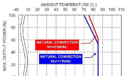
Derating Curve vs. Ambient Temperature MSD30USxxB xx=12/15/24/28/36/48/53 Connector Option : (-: JST)
