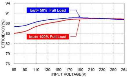
MSD30US24B Efficiency vs. Input Voltage
