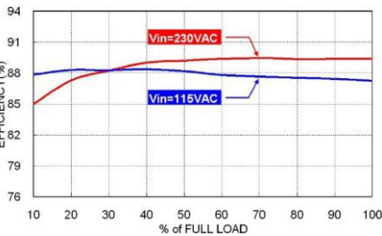
MSD30US24B Efficiency vs. Output Load
