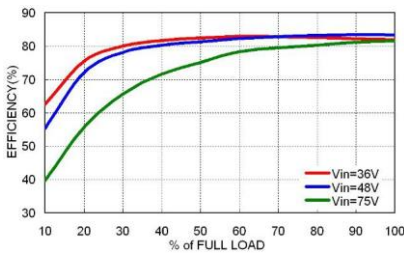
PDL06-48S05 Efficiency vs. Output Load
