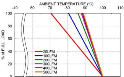
PDL06-48S05WM Derating Curve
