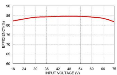
PDL06-48S05W Efficiency vs. Input Voltage
