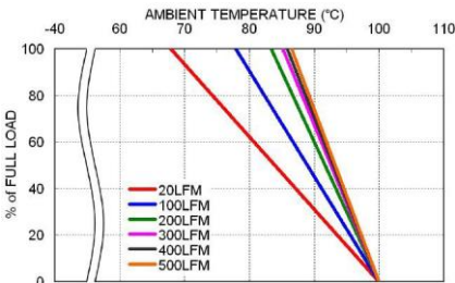
PDL06-48S05W Derating Curve
