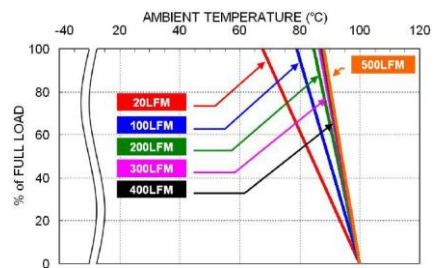
PDL09-24S12M Derating Curve
