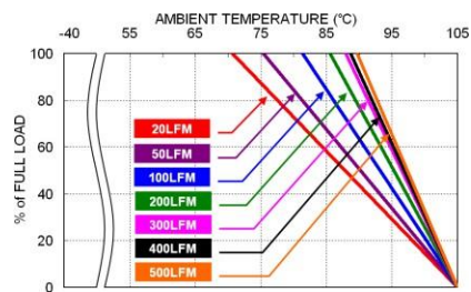
PDL12-48S05W Derating Curve With Recommended PCB Layout
