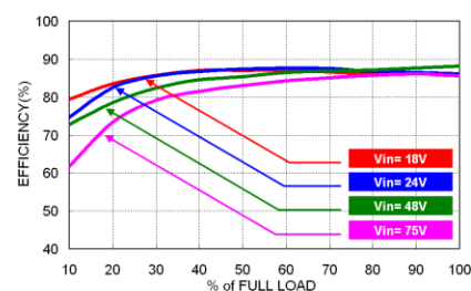
PDL12-48S05W Efficiency vs. Output Load
