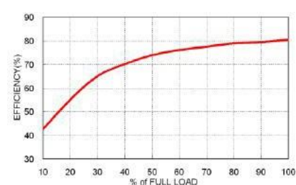
PDS02-48S05 Efficiency vs. Output Load
