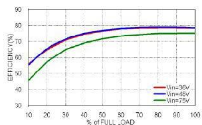
PFKC05-48S05 Efficiency vs. Output Load
