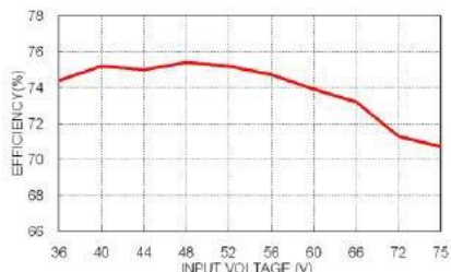
PMKC03-48S05 Efficiency vs. Input Voltage
