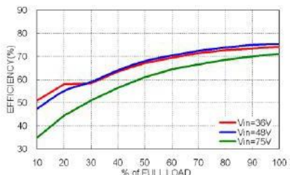
PMKC03-48S05 Efficiency vs. Output Load
