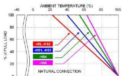
QAE100-24S05W Derating Curve with Heat-sink (See Thermal Considerations)
