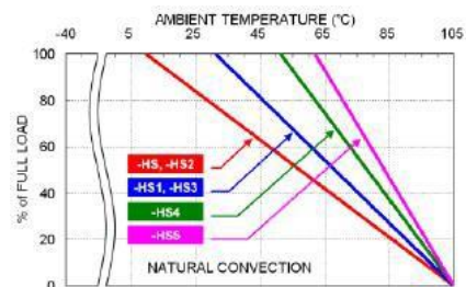
QAE150-48S05 Derating Curve with Heat-sink (See Thermal Considerations)
