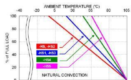
QAE150-24S05W Derating Curve with Heat-sink (See Thermal Considerations)
