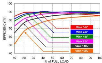
QAE40-72S05U Efficiency vs. Output Load
