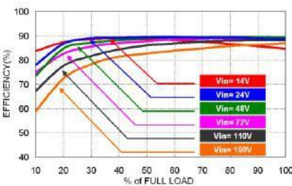
QAE60-72S05U Efficiency vs. Output Load
