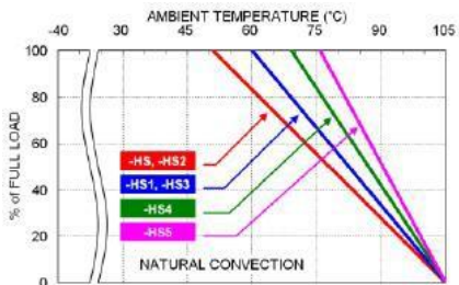
QAE60-72S05U Derating Curve with Heat-sink (See Thermal Considerations)
