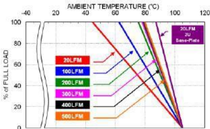
QAE60-72S05U Derating Curve (See Thermal Considerations)
