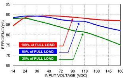
QAE60-72S05U Efficiency vs. Input Voltage
