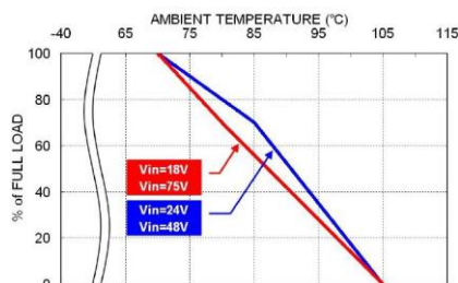
RCD15-48S05W Derating Curve
