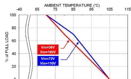
RCD15-110S05W Derating Curve
