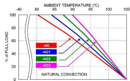
RCD15-24S05W Derating Curve With Heat-sink
