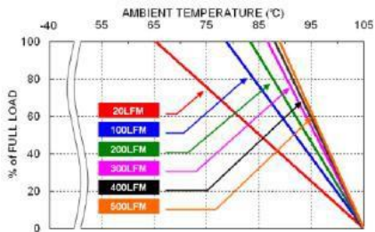
RCD20-48S05W Derating Curve
