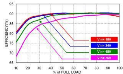
RCD30-48S05W Efficiency vs. Output Load
