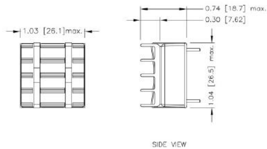
RCD30-□□□□W-HC1 7GA0117P01-F
