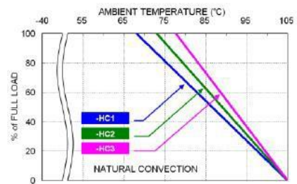
RCD30-48S05W Derating Curve with Heat-sink
