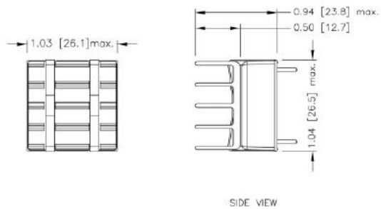
RCD30-□□□□W-HC2 7GA0118P01-F
