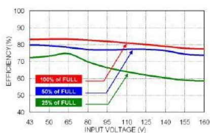
RDL03-110S05W Efficiency vs. Input Voltage
