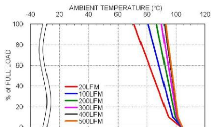
RED20-48S05W Derating Curve
