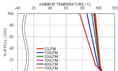
RED20-48S05W Derating Curve With Heat-sink
