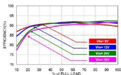
RED40-24S05W Efficiency vs. Output Load
