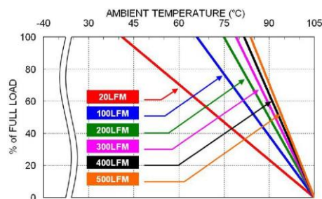
RHD40-110S05W Derating Curve
