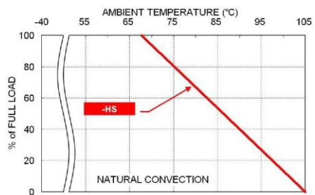
RHD40-110S05W Derating Curve With Heat-sink
