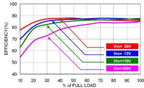
RHD40-110S05W Efficiency vs. Output Load
