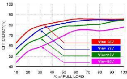
RHK03-110S24W Efficiency vs. Output Load
