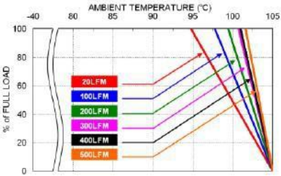
RHK03-110S24W Derating Curve
