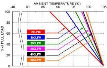
RHK06-110S12W Derating Curve
