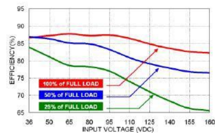
RHK06-110S12W Efficiency vs. Input Voltage
