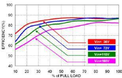
RHK06-110S12W Efficiency vs. Output Load
